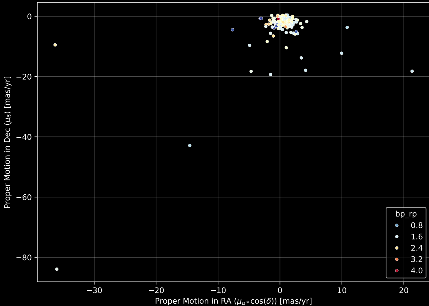
APOGEE DR17 Field: [173+04] Proper Motion Diagram (n= 189)
