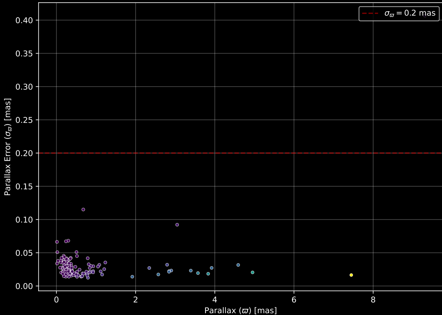
APOGEE DR17 Field: [173+04] Parallax Quality (n= 189)
