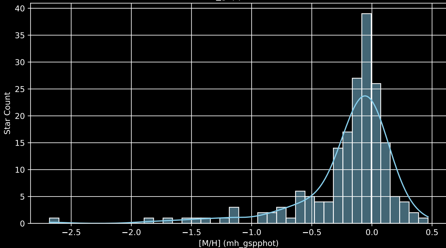
APOGEE DR17 Field: [173+04 [M/H] (mh_gspphot) (n= 187)
