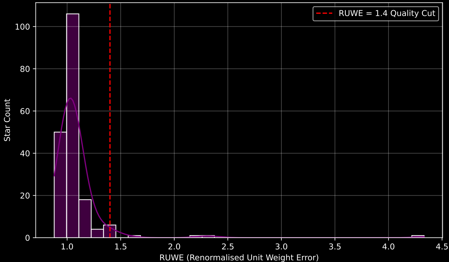
GAPOGEE DR17 Field [173+04] RUWE Distribution (n= 188)
