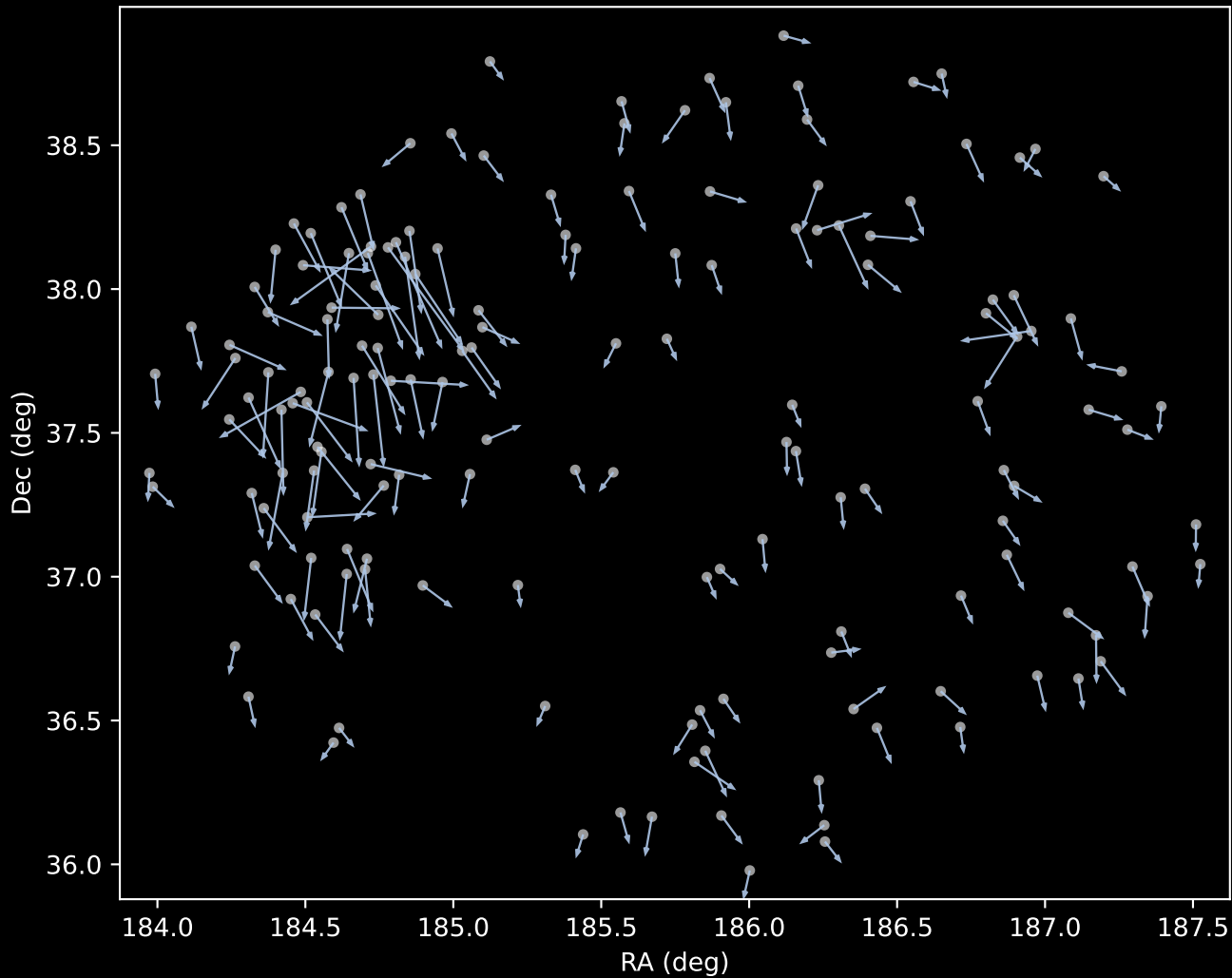
APOGEE DR17 Cluster 1 Proper Motion Vectors (n=161)
