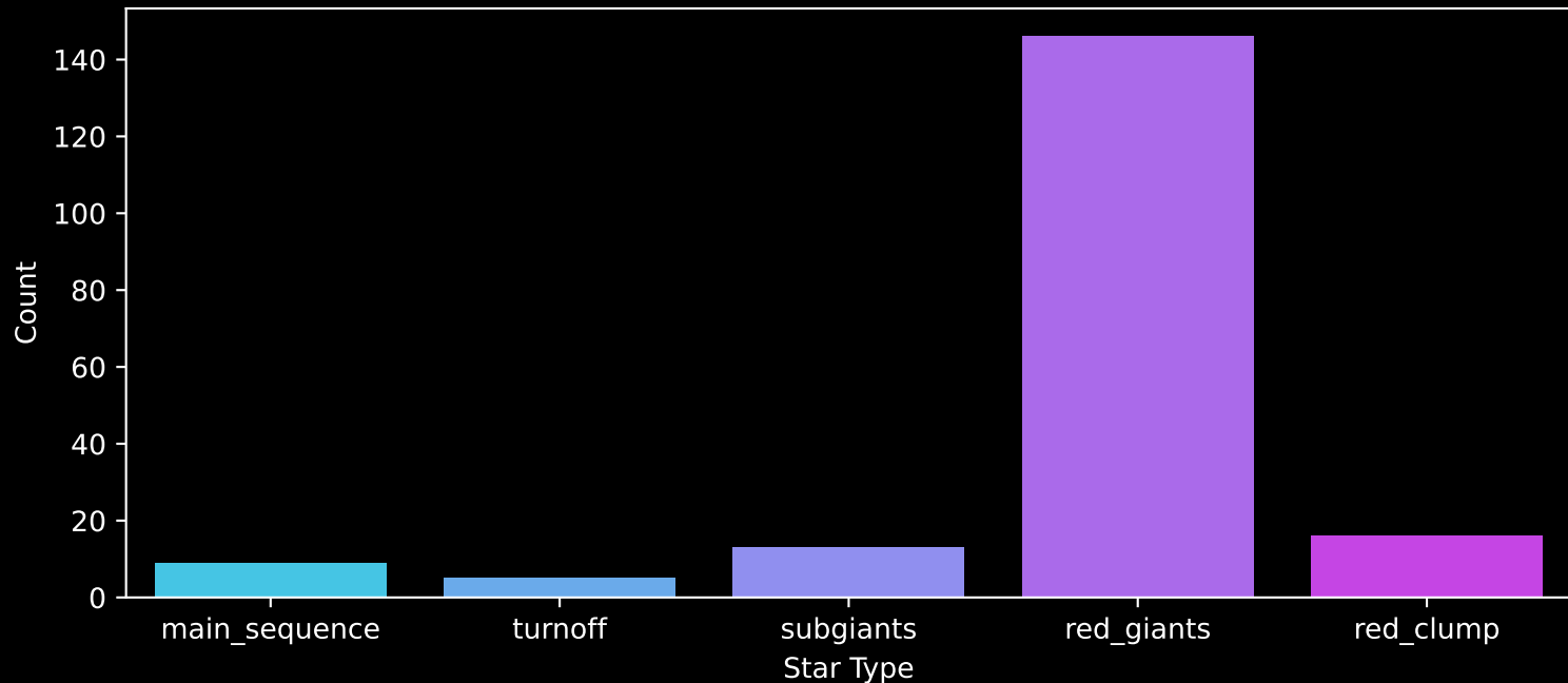
APOGEE DR17 Field: [173+04] Count plot of Star Type
